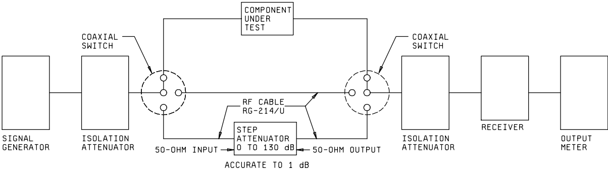
FIGURE 3. Alternate test circuit for rapid measurement.
