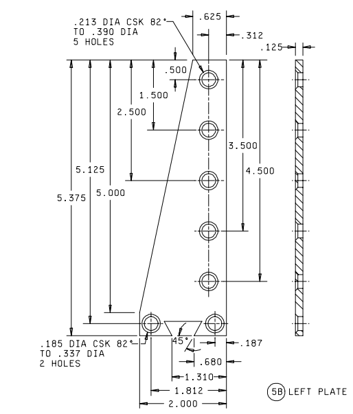
FIGURE 7. RF-dc insertion loss measuring equipment assembly - Continued.
